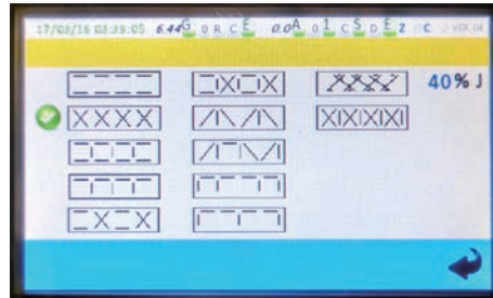
Touch panel display and 12 standard stitch patterns
